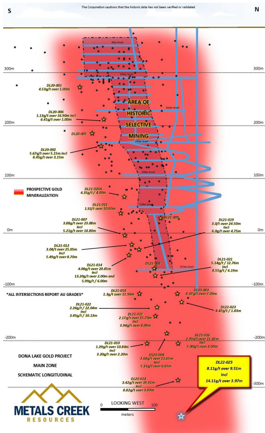
Figure 1. Schematic vertical long section of the Dona Lake Mine illustrating mined out portion and highlights of diamond drill results within Main Zone.
